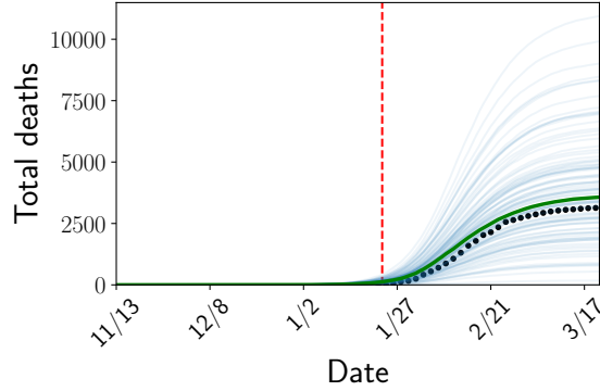
Figure 2: Simulated trajectories of the number of deaths over time in Hubei, China compared to the true number of reported deaths ( p_{\text{inf}} = 0.020 , t_0 = \text{November 15} ). Light blue lines are individual trajectories, green is the median, and the black dots are the number of reported deaths. The red dashed line represents the January 23 lockdown. The true number of reported deaths is contained within the simulated distribution and lies close to the median (Pearson r = 0.998 ).
