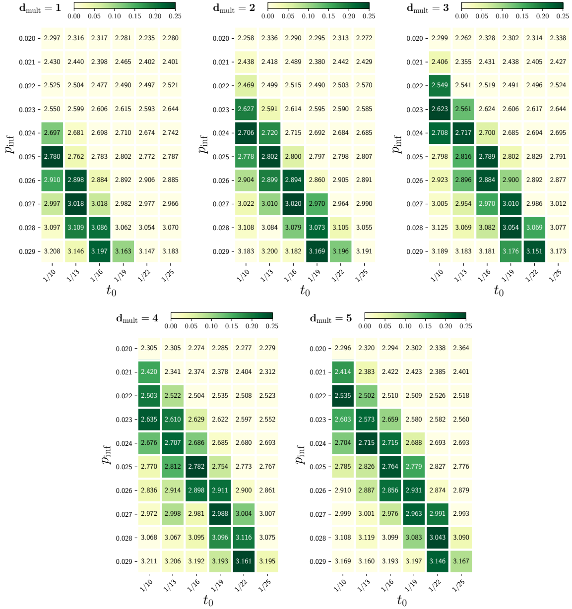
Figure 7: r_0 during the exponential growth (pre-lockdown) phase in Lombardy as a function of p_{\text{inf}} ( y axis) and t_0 ( x axis). From left to right, top to bottom: a mortality multiplier d_{\text{mult}} relative to China of 1, 2, 3, 4, 5. Colors indicate goodness of fit of the parameter settings to the true number of reported deaths on March 21 in Lombardy, with darker cells indicating a better fit. The plausible range for r_0 is 2.50-3.20.
