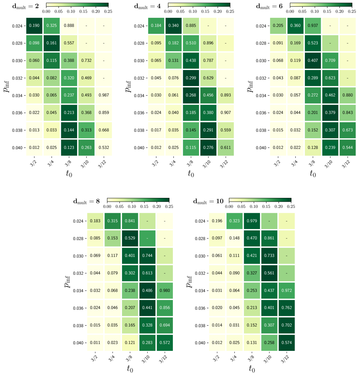
Figure 7: Estimated fraction of symptomatic infections that become documented in Uttar Pradesh as a function of p_{\text{inf}} ( y axis) and t_0 ( x axis). Each plot corresponds to a higher mortality multiplier d_{\text{mult}} . Darker cells indicate better goodness of fit of the corresponding parameter settings to the true number of reported deaths on 10 April. A broad range of parameter combinations fit the data well, giving a very wide plausible range of 11.33%–99.54% for the documentation rate. This wide range is likely due to the small number of deaths that have been reported so far in the state, making precise parameter fits challenging to achieve.
