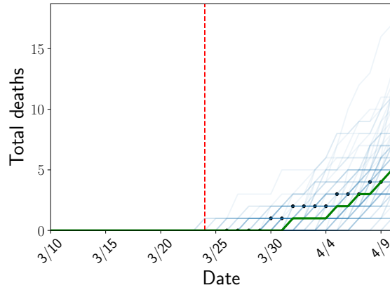
Figure 9: Simulated trajectories of deaths in Uttar Pradesh ( p_{\text{inf}} = 0.036 , t_0 = 10 March, d_{\text{mult}} = 6 ). Dotted black lines represent true reported COVID-19 deaths. Blue lines are independent simulations and the green line is the median of the simulations. The red dashed line marks the nationwide lockdown instated on March 24. The true number of reported deaths is well contained within the simulated trajectories and lies close to the median (Pearson r = 0.917 )
