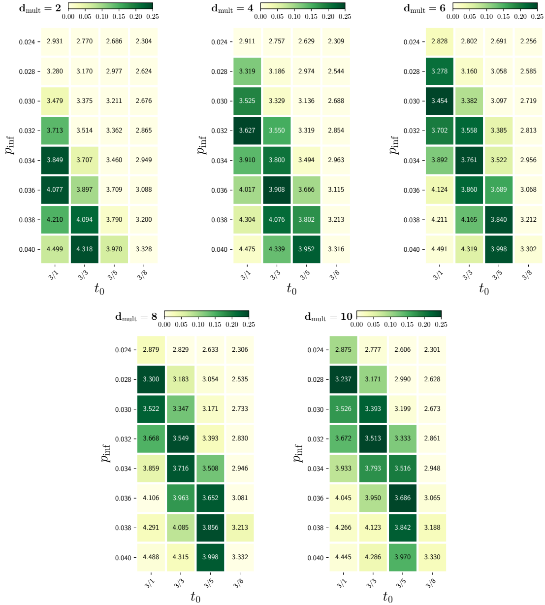
Figure 6: Estimated values of R_0 for Maharashtra during the pre-lockdown phase as a function of p_{\text{inf}} ( y axis) and t_0 ( x axis). Each plot corresponds to a higher mortality multiplier d_{\text{mult}} . Darker cells indicate better goodness of fit of the corresponding parameter settings to the true number of reported deaths on April 10. A broad range of parameter combinations fit the data well, giving a plausible range of 3.00–4.21 for R_0 .
