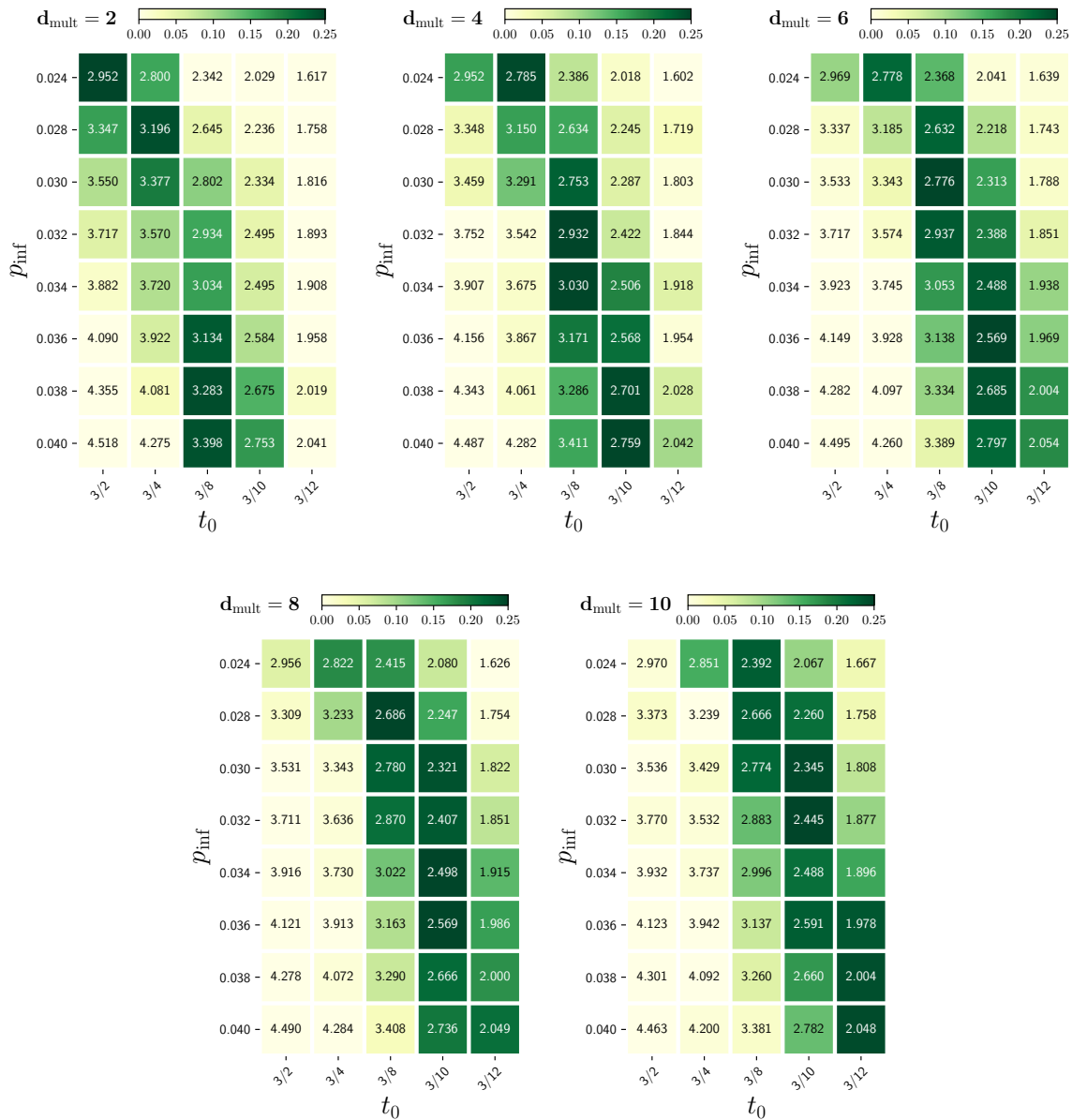
Figure 8: Estimated values of R_0 for Uttar Pradesh during the pre-lockdown phase as a function of p_{\text{inf}} ( y axis) and t_0 ( x axis). Each plot corresponds to a higher mortality multiplier d_{\text{mult}} . Darker cells indicate better goodness of fit of the corresponding parameter settings to the true number of reported deaths on 10 April. A broad range of parameter combinations fit the data well, giving a plausible range of 1.97–3.46 for R_0 .
